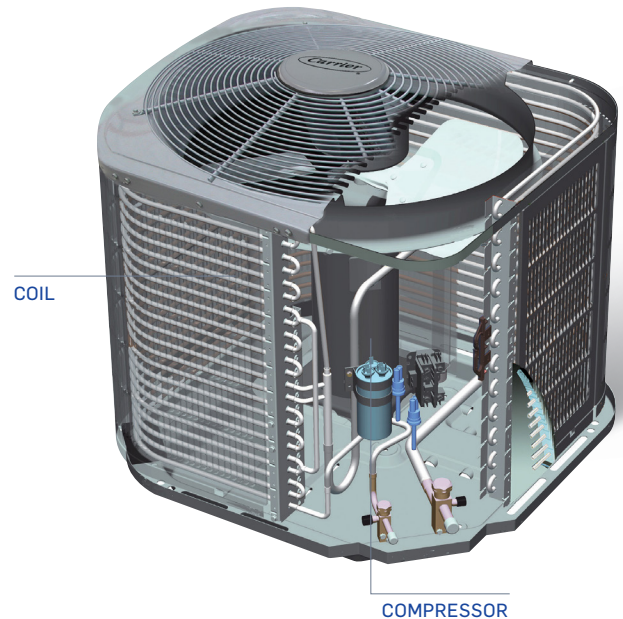
PERFORMANCE™ 16 AIR CONDITIONER
